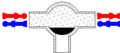
3-way (0°-90°-180°)
