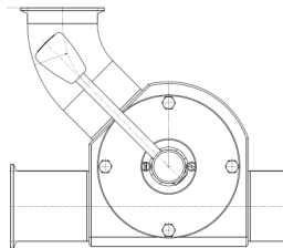
Venturi (powder control)
