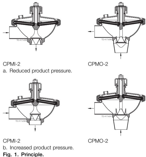
Fig. 1. Principle.
